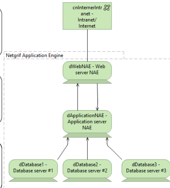
Picture 4 – Technological architecture of the Netgrif Application Platform
